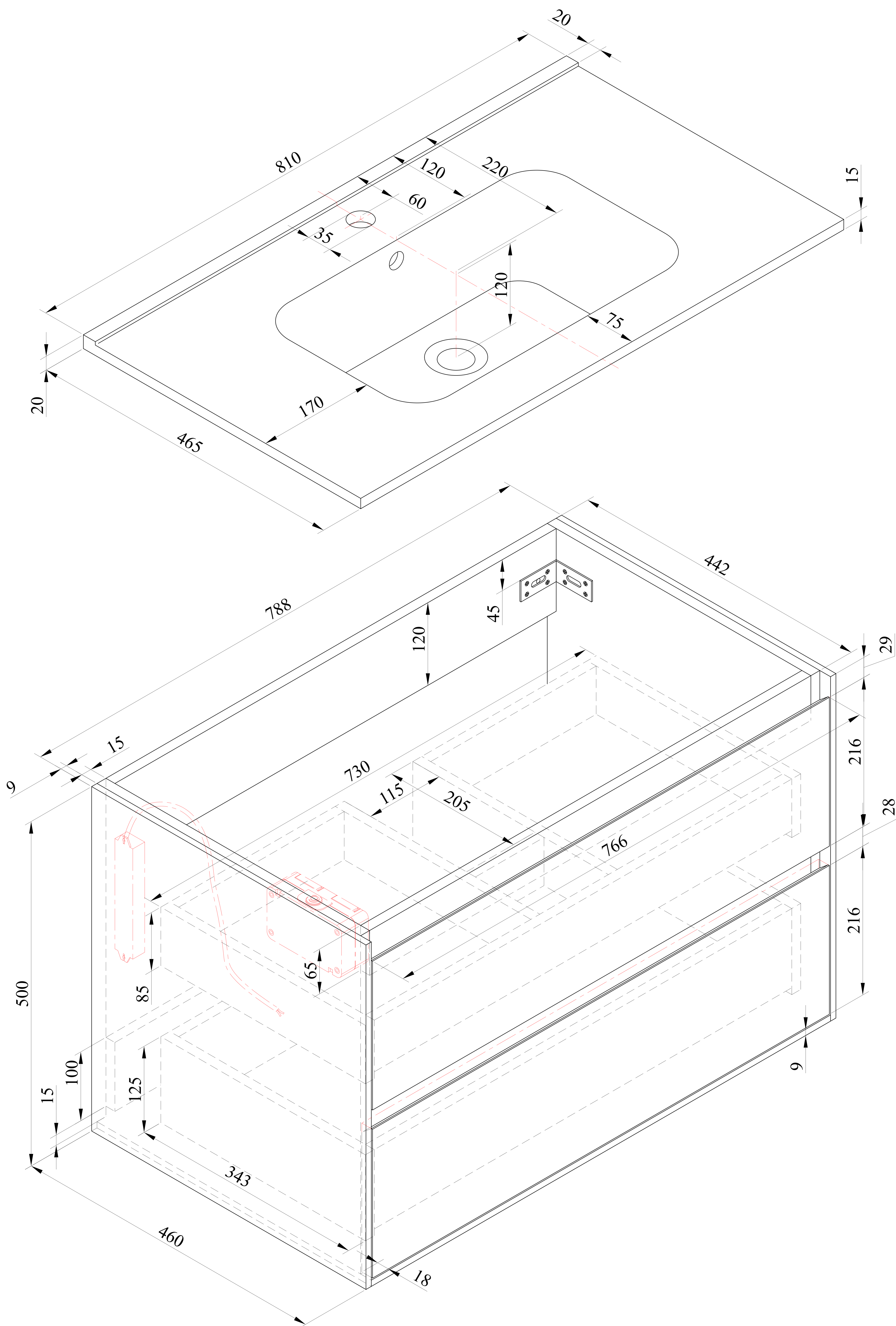
LATTNAD 80
