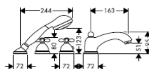
Carlton 17461XXX
