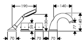
Starck 10461XXX
