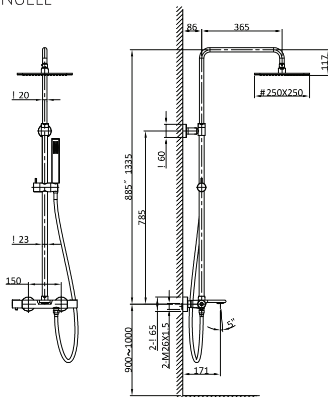
Installation drawing
