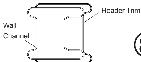
Wall Channel Assembly (Painted)
