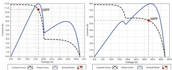
Figure 1-3 Multi-MPP kurva
