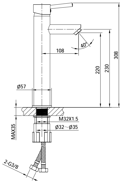
Installation drawing
