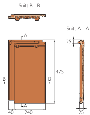
TURMALIN
