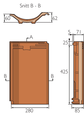
NORTEGL
