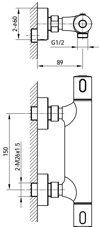
Installation drawing
