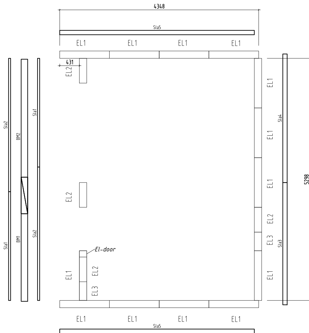
Wall panel plan
